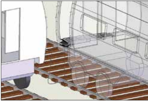
Figure 1-4 – Turn transfer bridge 90° and carefully unfold top section (one fold) as shown.
